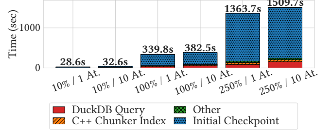
Figure 12: Execution time breakdown on 10 %, 100 %, and 250 % versions of The Pile with 1 and 10 attributes (3 run average).
