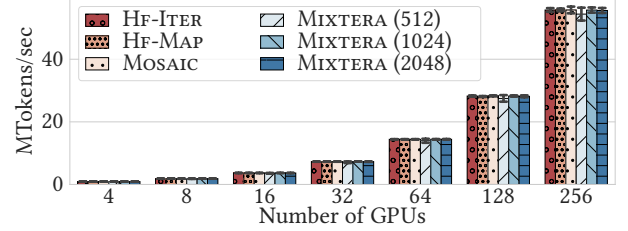
Figure 8: Data loader throughput when increasing the number of data parallel nodes.
